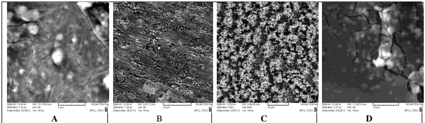
Figure 6: (a,b) Micrographs of metal surface after removal of Biofilm showing Oxide film and rough surface (c,d) tubercle surface and biofilm in tubercle surface
