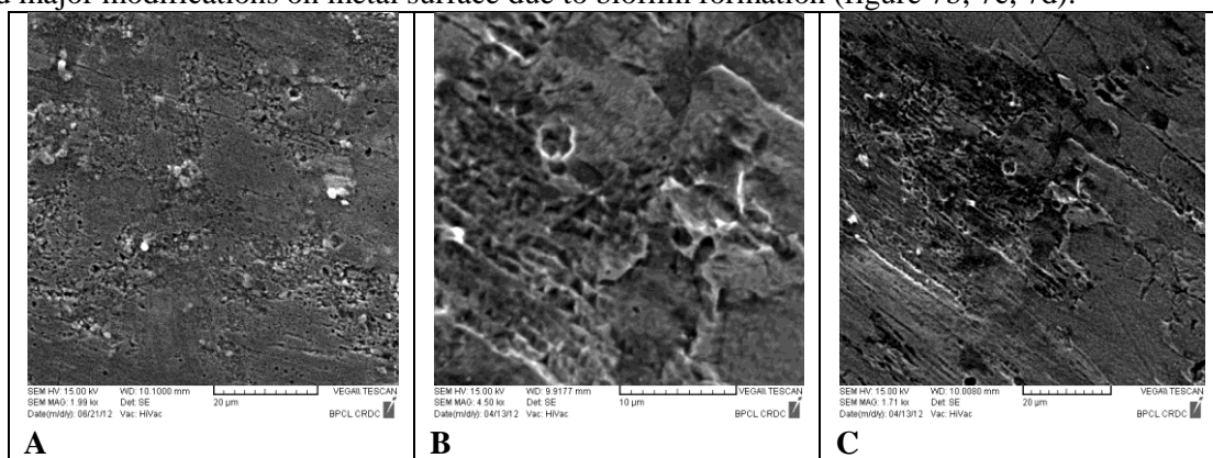
Figure 7: (a) Carbon steel metal surface after exposure to sterile media (b,c) Micrograph of pits on the metal surface exposed to SRB medium for 24 days
