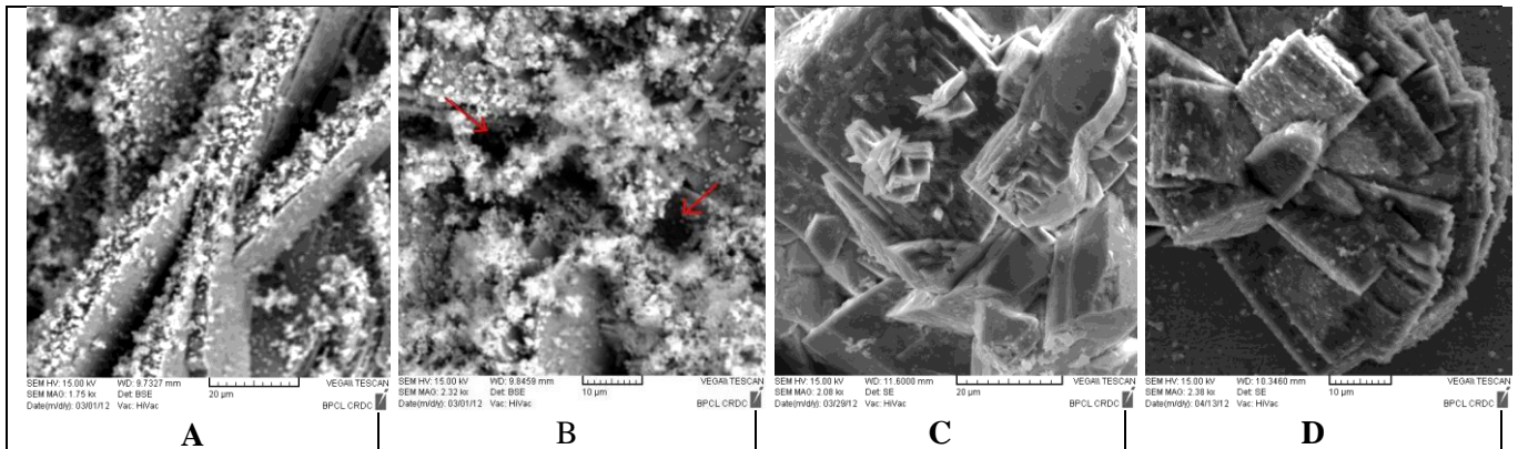
Figure 4: (a,b) Amorphous biofilm (arrows pointing voids within the biofilm) (c,d) crystalline biofilm formation on metal surface
