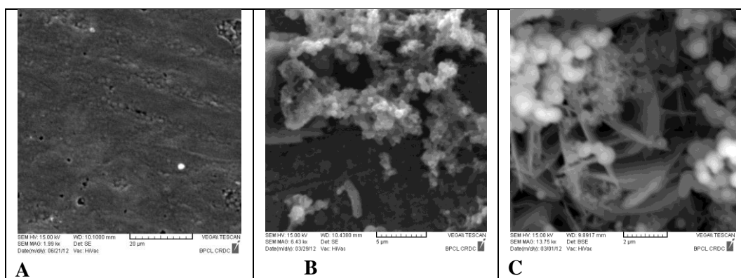
Figure 5: (a) Control showing no biofilm formation after 40 days (b) Dense biofilm with SRB embedded and (c) Spores are observed in biofilm after 24 days exposure
