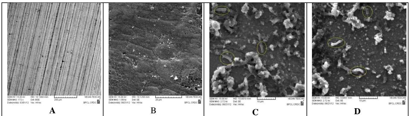
Figure 3: (a) Carbon steel metal surface before immersion test; (b) Metal surface exposed to sterile media showing no biofilm formation after 48 hours; (c,d) SRB attached on the surface of carbon steel after 48 hour exposure
