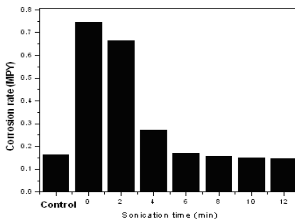
Figure 8: Effect of sonication on corrosion rate
