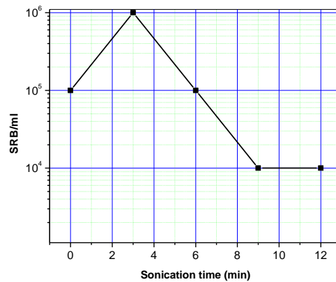
Figure 2: Effect of sonication on SRB count of aeration basin inlet sample
