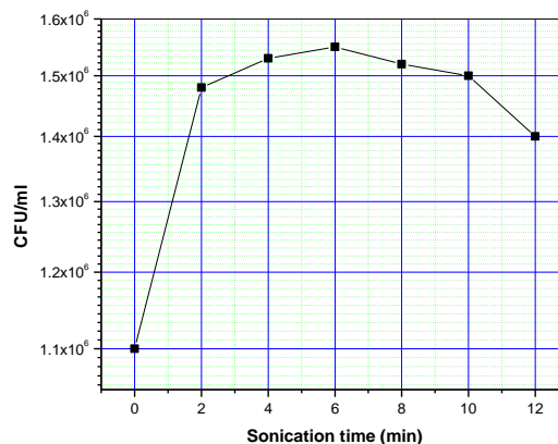
Figure 1: Effect of sonication on microbial count of aeration basin inlet sample
