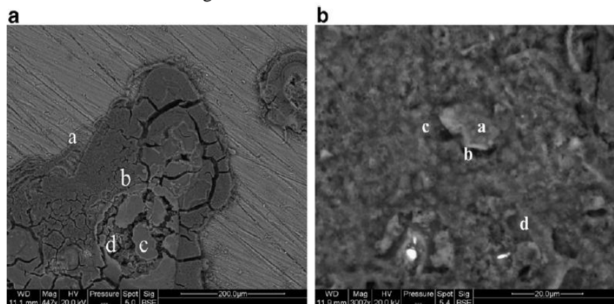
Figure 3: SEM micrographs of (a) Mg and (b) Mg-6SiC after corrosion in 1M NaCl solution [21]
