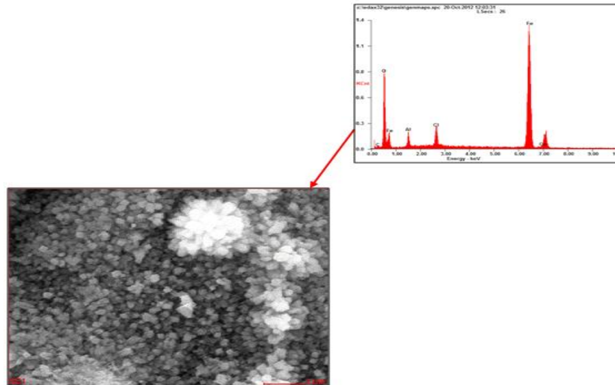
Figure 6: SEM and EDAX of full frame of the specimen 10AFel.0Co1100(1) showing nano size particles after corrosion in 1N HCl at 20000X magnification [26]
