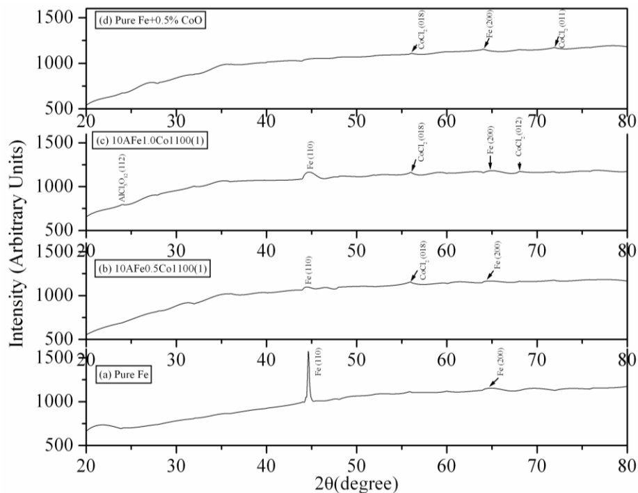
Figure 5: XRD patterns of the corroded surfaces of (a) Pure Fe (b) 10AFe0.5Co1100(1) (c) 10AFe1.0Co1100(1) and (d) Pure Fe+0.5% CoO specimens respectively [26]
