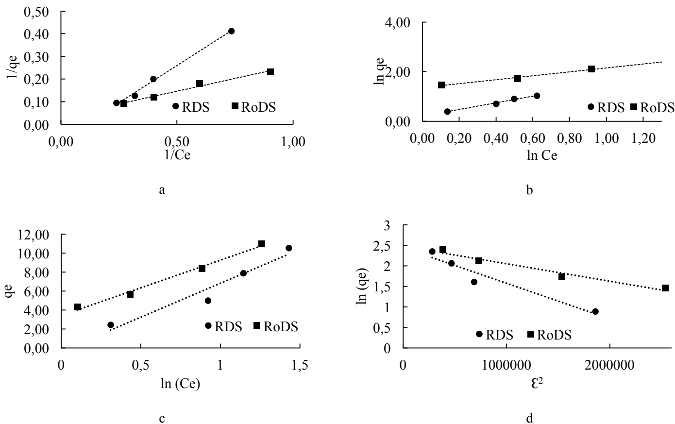
Figure 9: Langmuir (a), Freundlich (b), Temkin (c) and Dubinin (d) isotherm models plots of MB adsorption onto RDS and RoDS
