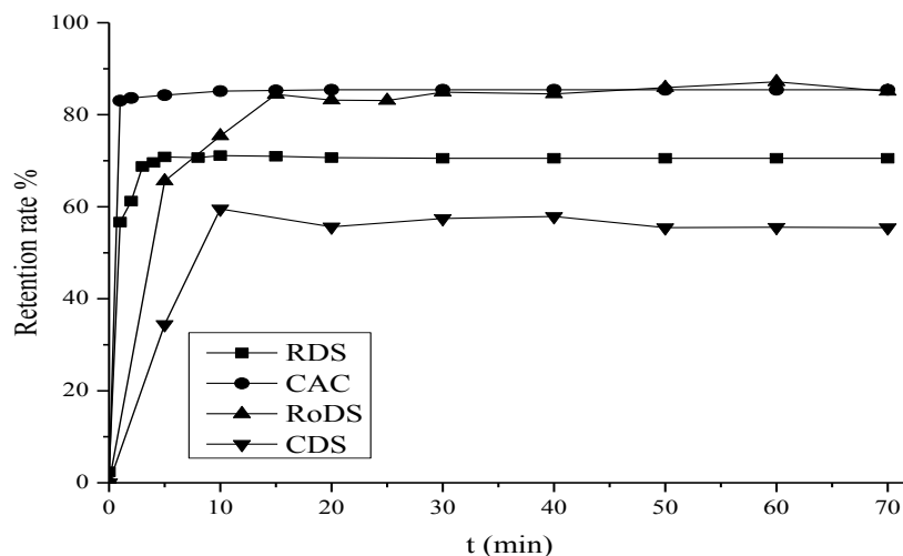
Figure 6: Adsorption kinetics of MB onto RDS, RoDS, CDS and CAC
