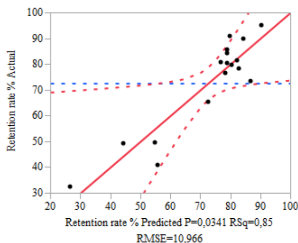
Figure 3: Predicted versus experimental MB Removal (%R) of RDS
