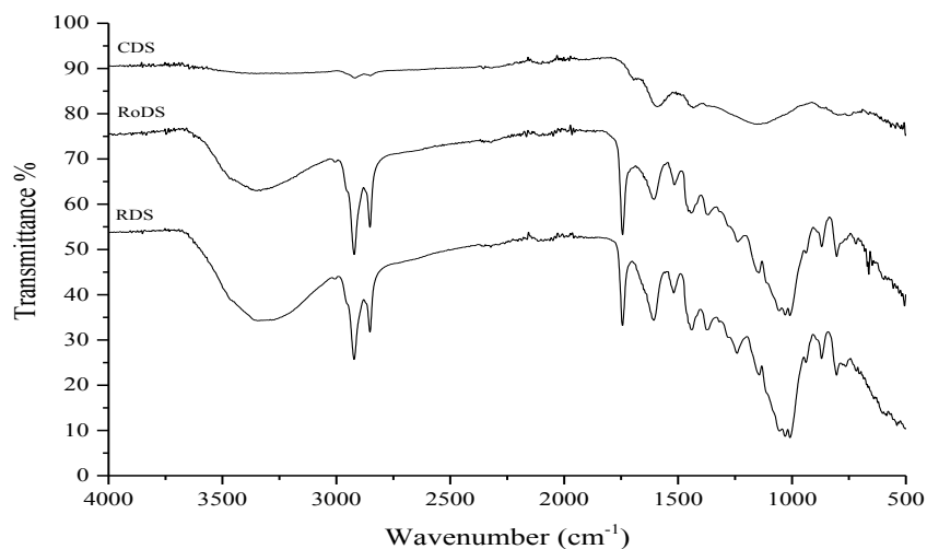
Figure 7: Infrared spectra of RDS, RoDS and CDS
