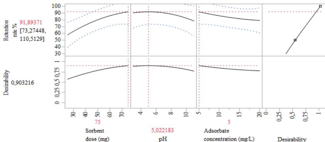
Figure 4: Prediction profiler outputs of JMP®11 software after maximization of the desirability
