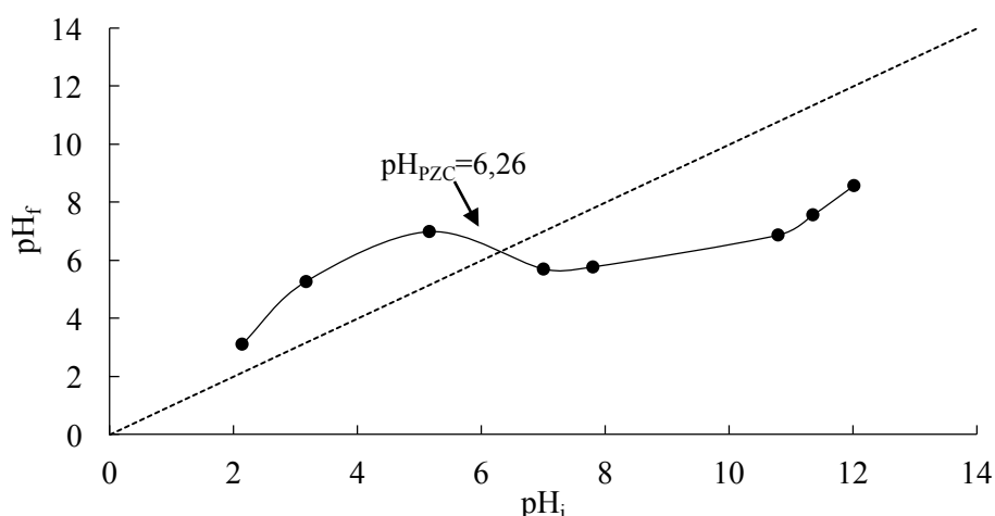
Figure 2: Titration curve ( pH_f=f(pH_i) ) obtained in NaCl 0.1M as supporting electrolyte
