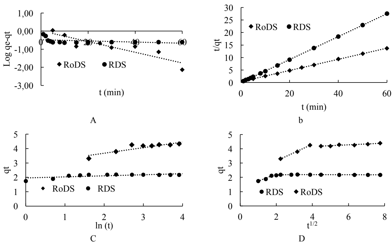
Figure 8 : Pseudo-first-order (a), pseudo-second-order (b), Elovich (c) and intra-particle diffusion (d) kinetic models of MB adsorption onto RDS and RoDS
