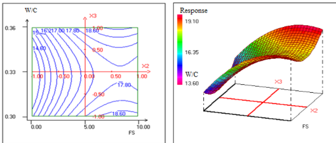
Figure 4: Variation of the compressive strength in the plane: W/C ratio, silica fume content with cement content = 62.92%
