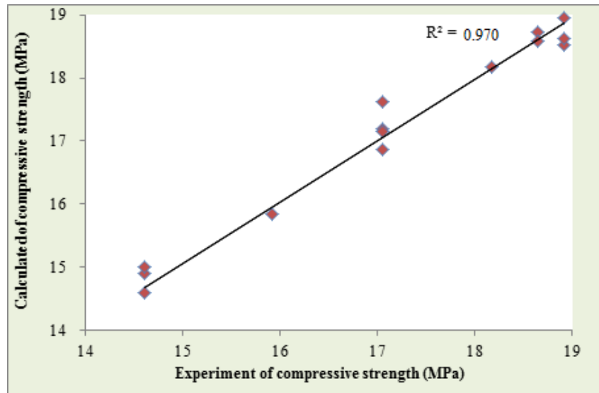
Figure 3: Comparative between theoretical and experimental results
