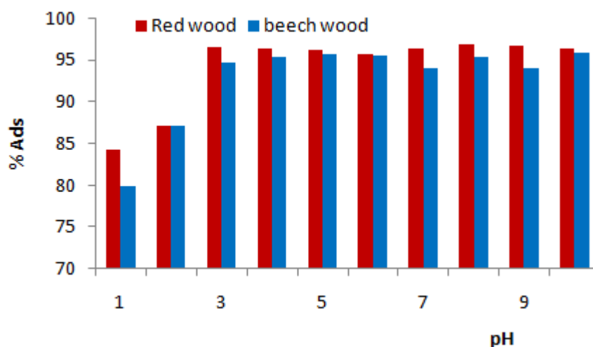
Figure 6: Variation of fixation percentage (% Ads) as a function of pH
