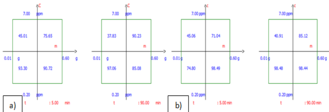
Figure 14: Diagram of the percentages of adsorption as a function of the interactions between factors X 1 , X 2 , X 3 a) Red wood, b) beech wood
