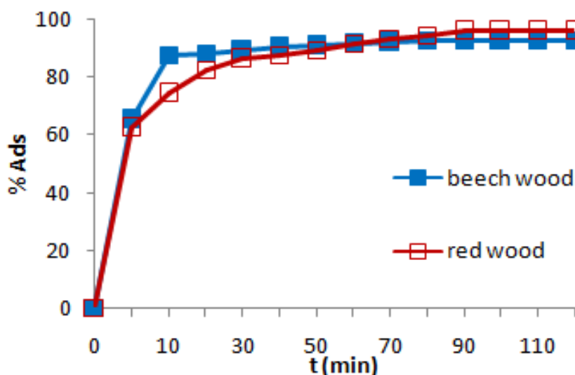
Figure 8: Variation of fixation percentage (%Ads) as a function of time contact
