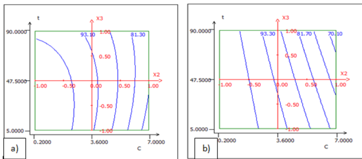
Figure 15: Variation of % Ads in 2D in the plan (c, t) a) red wood, b) beech wood (Fixed Factors: m = 0.305 g, \text{pH} = 2 )
