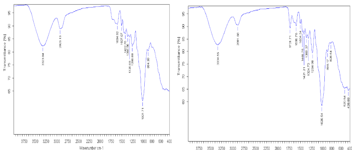
Figure 3: Infrared spectrum of red wood sawdust Figure 4: Infrared spectrum of beech wood sawdust
