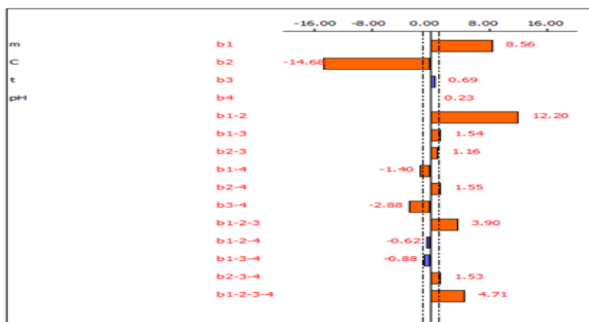
Figure 12: The factors effect's graph for methylene blue on red wood sawdust
