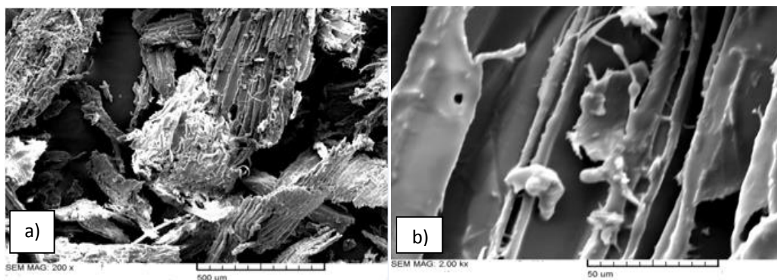
Figure 1: SEM micrograph of red wood sawdust: Enlargement a: x 200 ; b: x 2000
