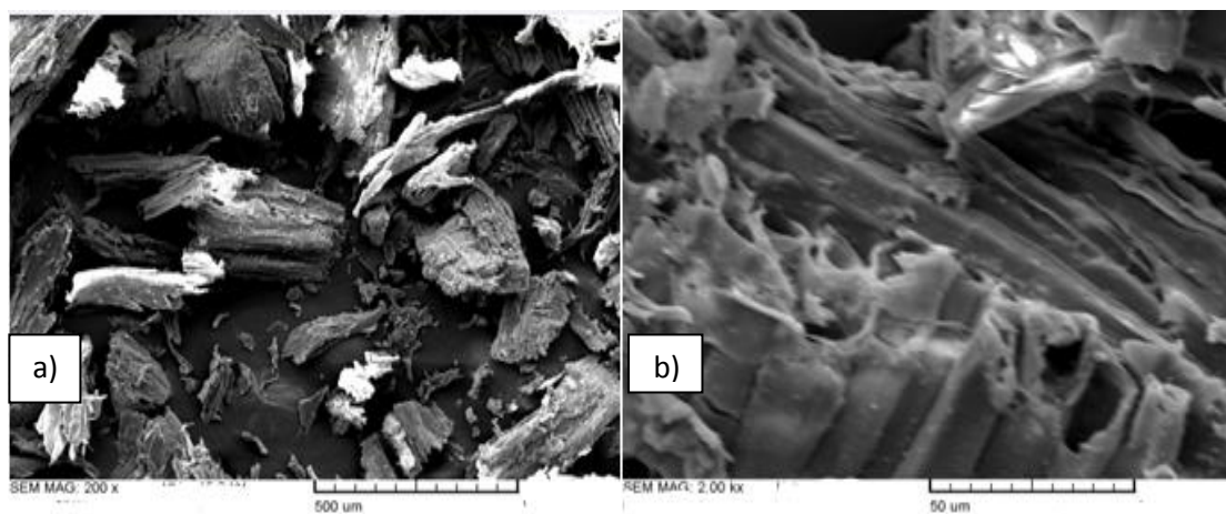
Figure 2: SEM micrograph Beech wood sawdust: Enlargement a: x 200; b: x 2000
