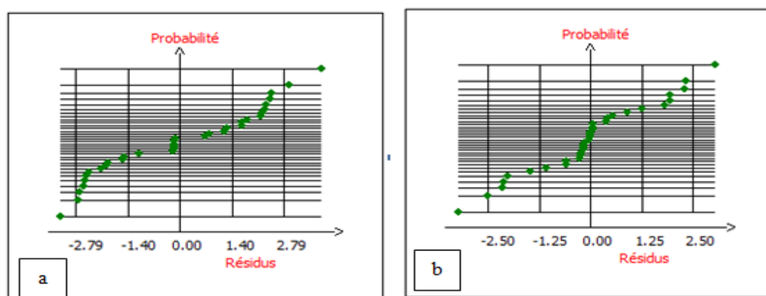
Figure 11: Study of residues a) Red wood , b) beech wood
