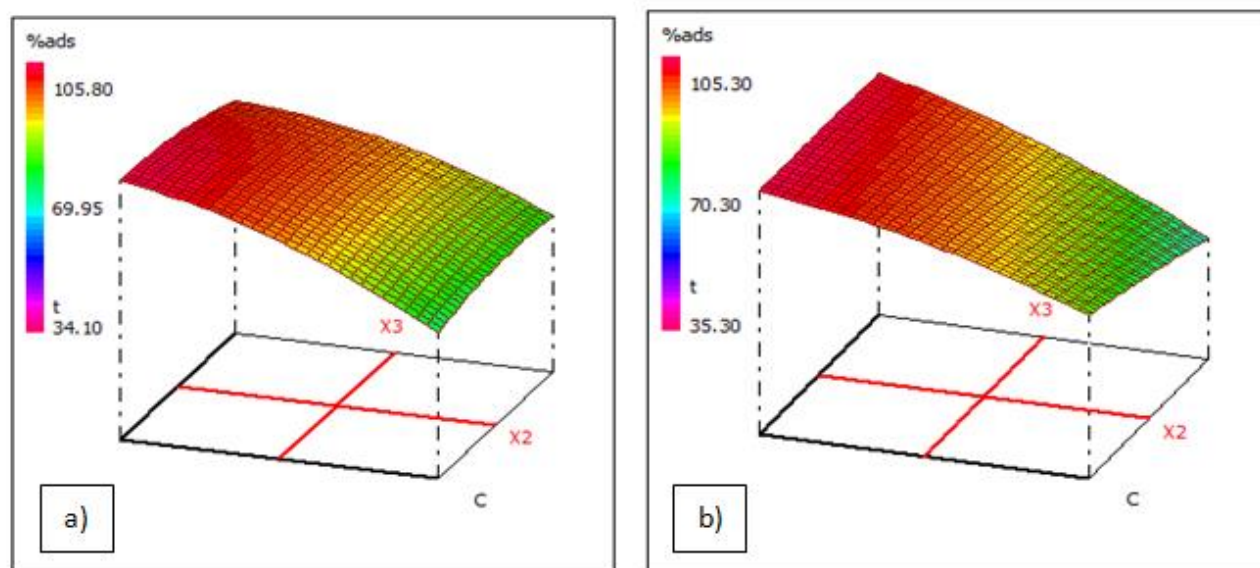
Figure 16: Variation of % Ads in 3D in the plan (c, t) a) red wood, b) beech wood (Fixed Factors: m = 0.305 g, \text{pH} = 2 )
