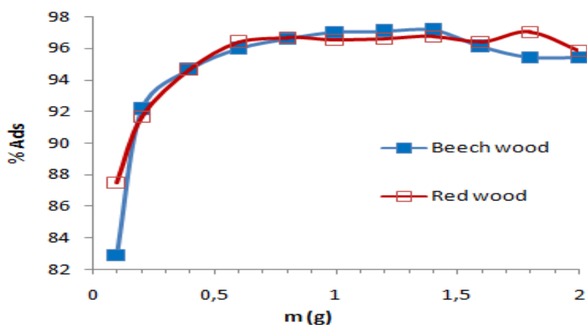
Figure 5: Variation of fixation percentage (% Ads) as a function of the mass (m)
