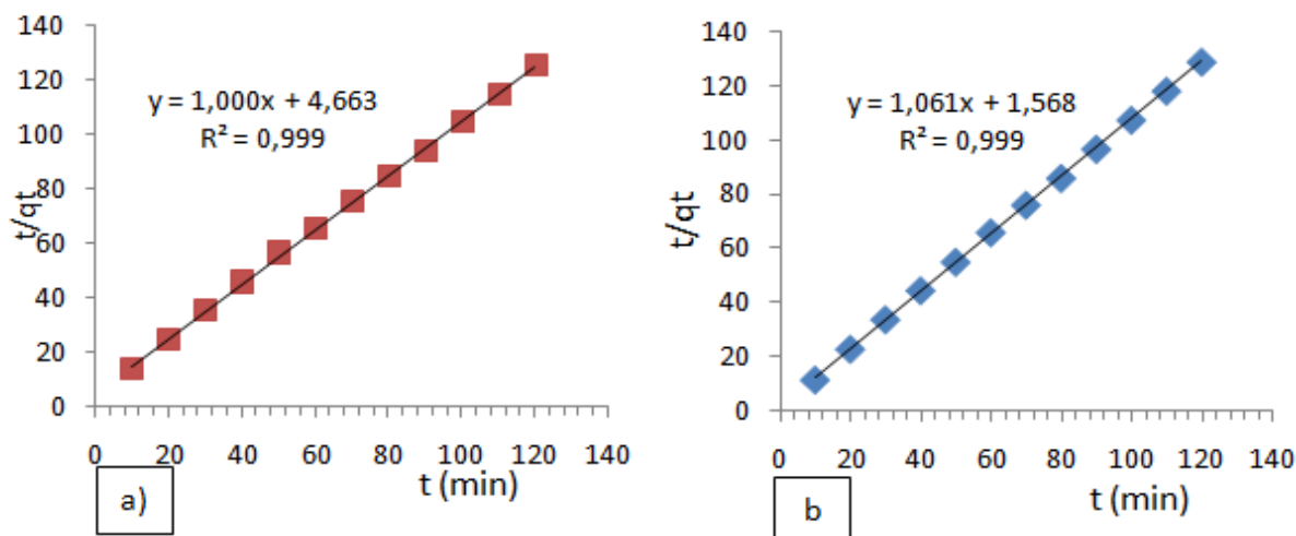
Figure 10: Second-order model a) Red wood b) beech wood
