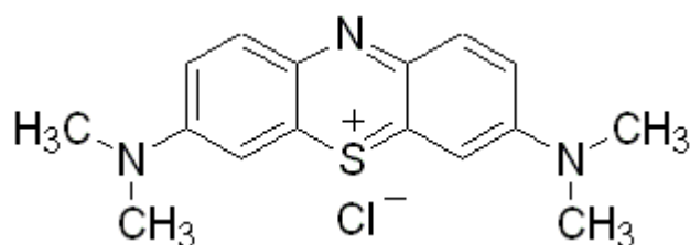
Molecular Structure of Methylene Blue
