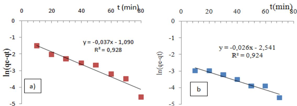
Figure 9: First order model: a) Red wood b) beech wood
