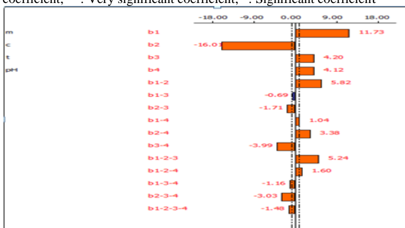
Figure 13: The factors effect's graph for methylene blue on beech wood sawdust
