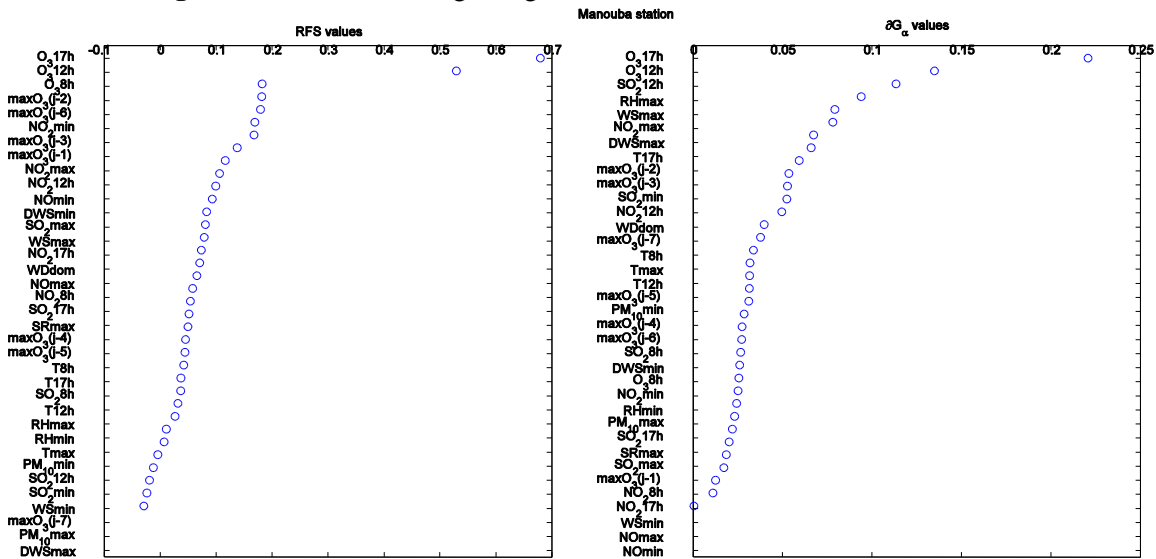
Figure 4: Variable ranking using RFS and \partial G_{\alpha} scores for Manouba station
